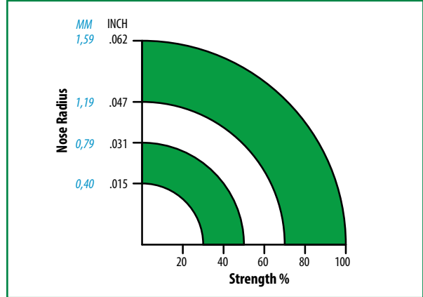
Figure 34c Relative Strength for Various Insert Radii
