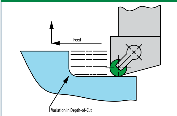
Figure 61c Multiple Passes at Varying Depths of Cut with Regular Wear
