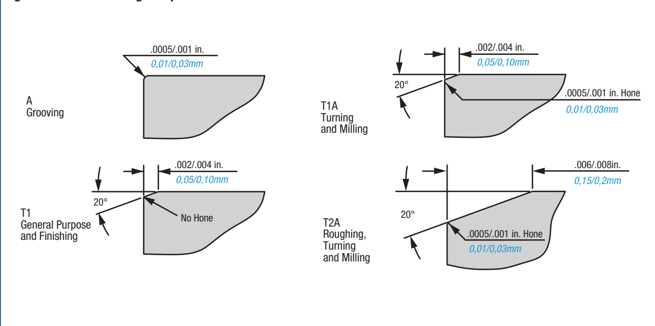
Figure 24 – Standard Edge Preparations
