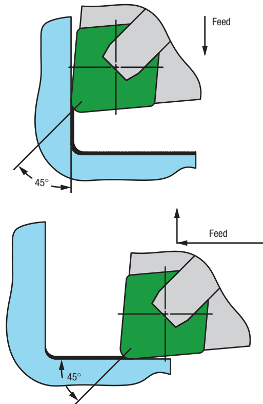
Figure 47 – Ceramic Method
