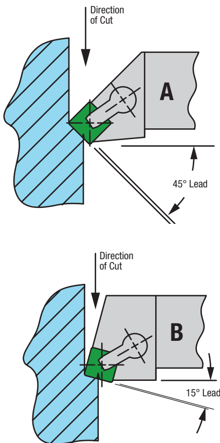
Figure 18 – Lead-Angle Effect
