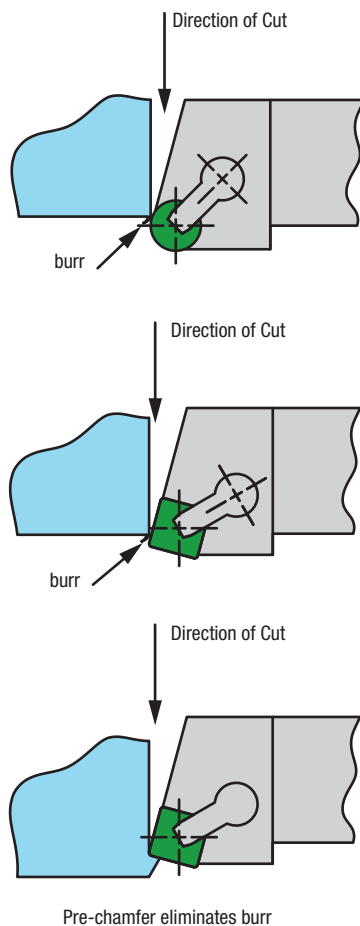
Figure 32 – Pre-Chamfer to Eliminate Burrs
