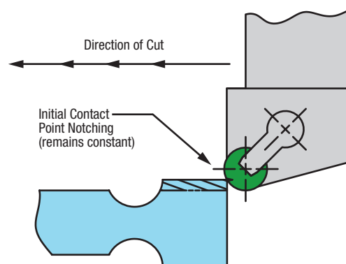
Figure 27 – Straight Facing
