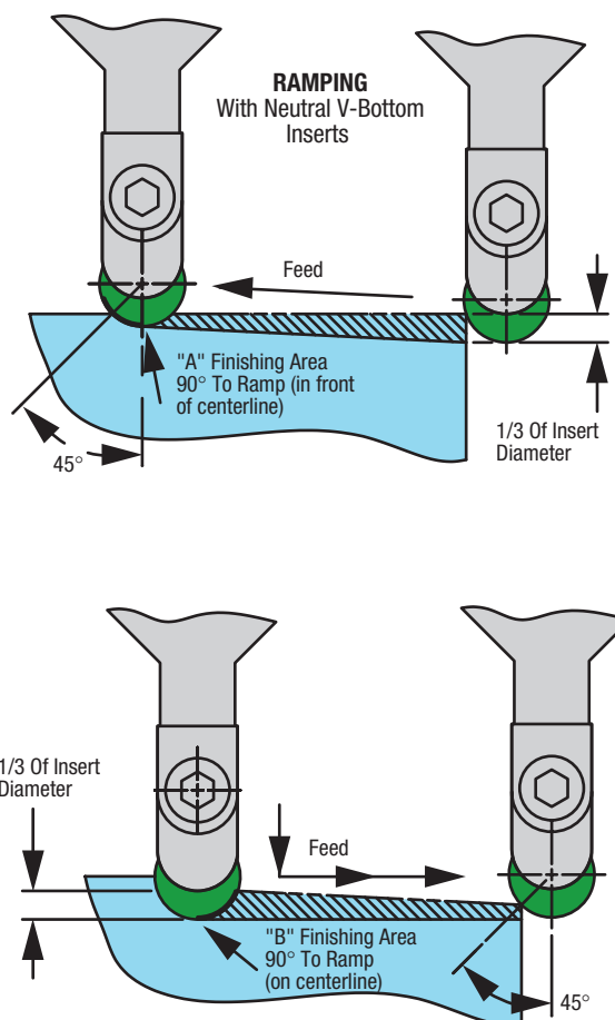
Figure 38 – Ramping/Positive Inserts/RPGN-RCGN
