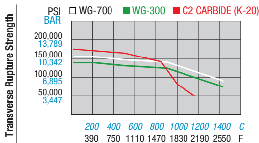
Figure 5 – Relative Strength at Elevated Temperatures
