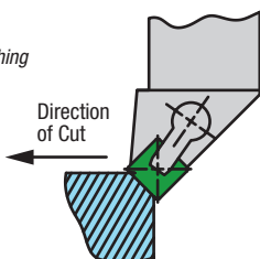
Figure 26 – Chamfering Techniques
